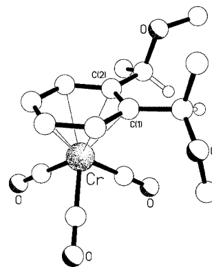
Figure 3. The molecular structure of 12 .
