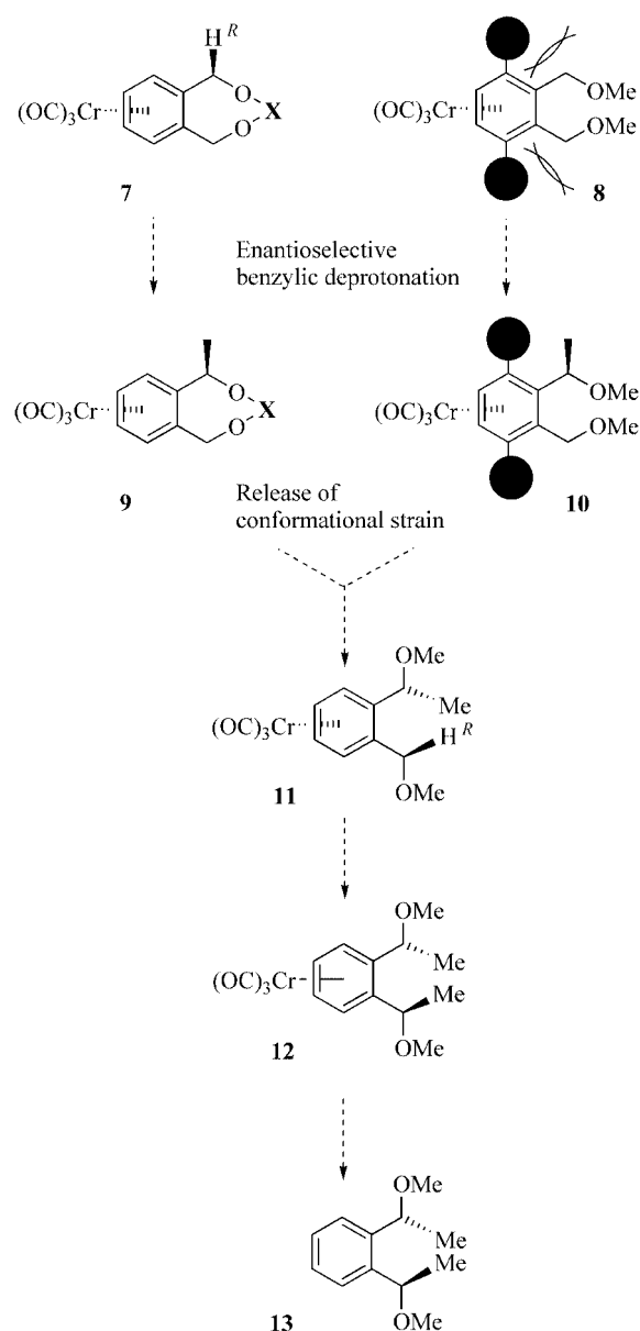
Figure 1. Two approaches to conformational control in tricarbonylchromium(0) complexes of ortho -substituted arenes.
